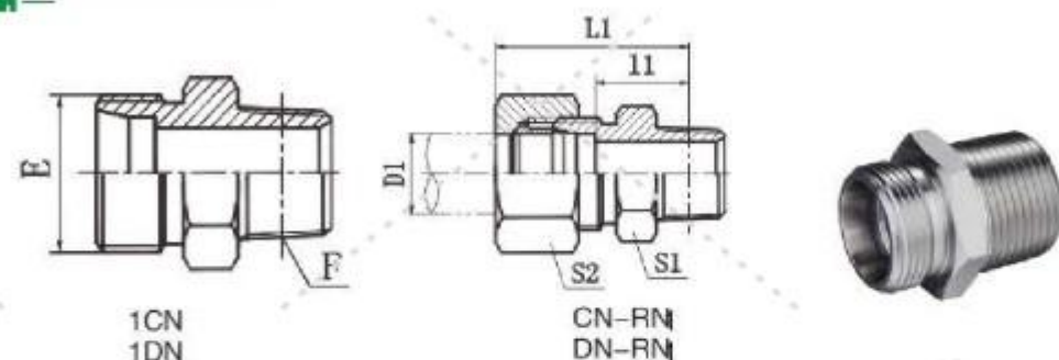
布锥管外螺纹 NPT MALE
