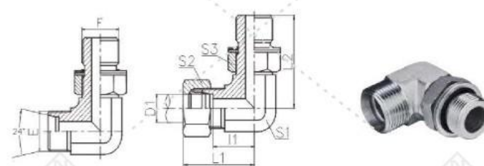
90° 弯英管螺纹可调向O形圈密封柱端 90° ELBOW BSPP THREAD ADJUSTABLE STUD ENDS WITH O-RING SEALING
