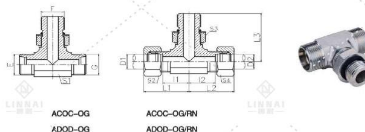
美制螺纹可调向O形圈密封柱端分支三通 UN、UNF THREAD ADJUSTABLE STUD ENDS WITH O-RING SEALING BRANCH TEE
