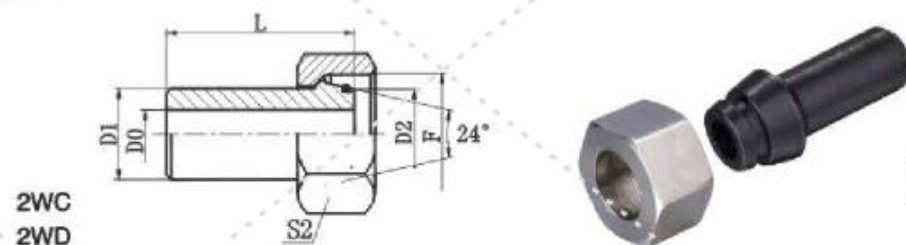
焊接接头 WELD FITTINGS
