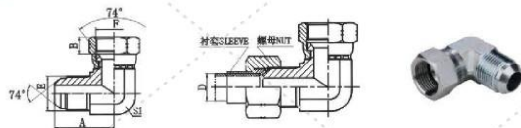
90° 弯美制JIC外螺纹74° 外锥/JIC内螺纹74° 内锥 90° ELBOW JIC MALE 74° CONE/ JIC FEMALE 74° SEAT
