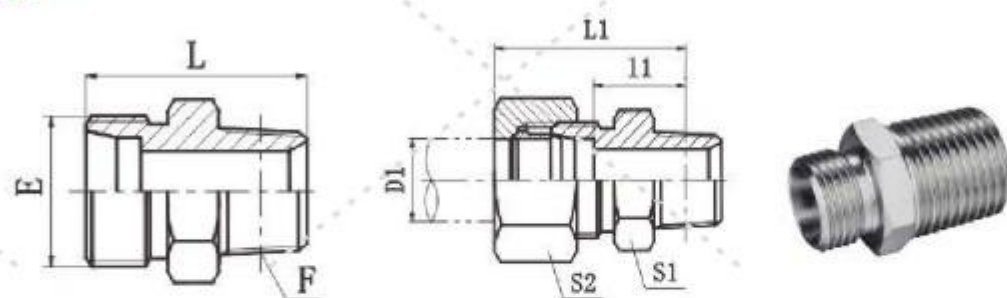
英锥管外螺纹 BSPT MALE
